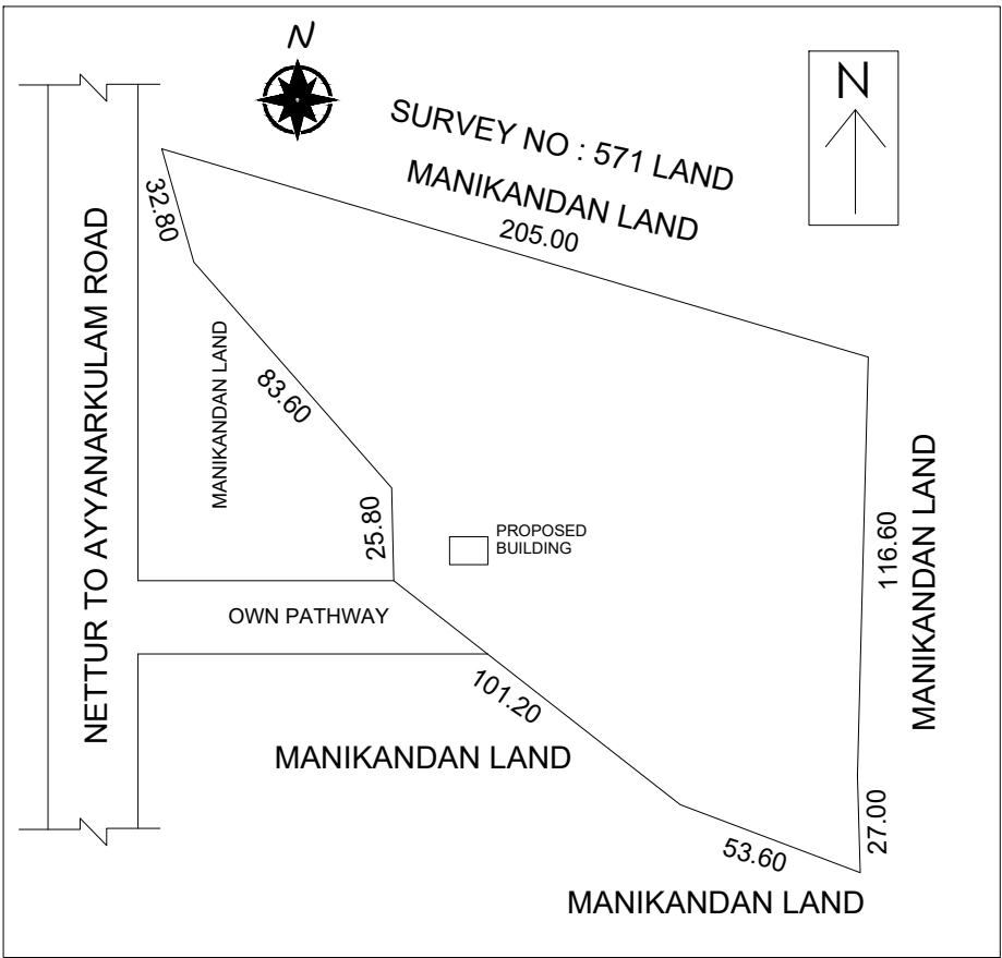
SITE PLAN ( SCALE:- 1:800 )
