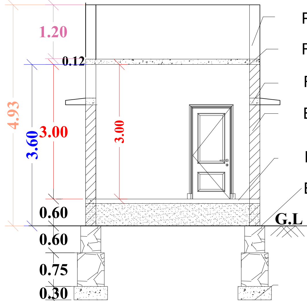
"SECTION "AB"
