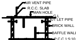
SECTION ON SEP.TANK
