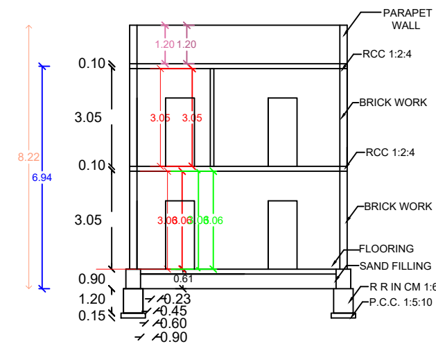
SECTION AB
