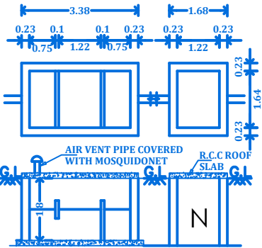
PLAN&SECTION OF SEPTIC TANK 'U' TRAP PROVIDED
