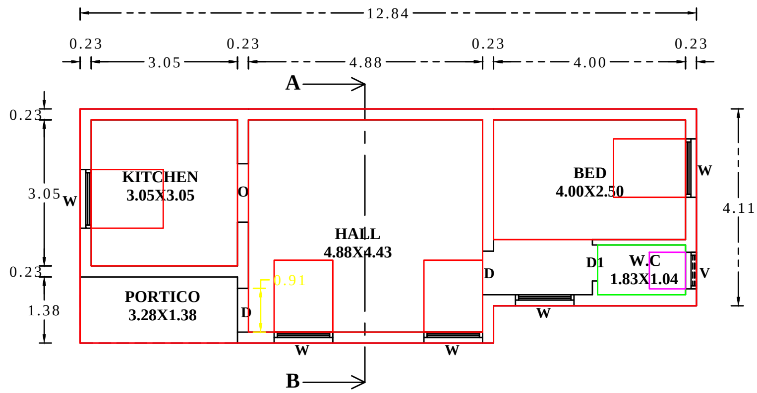
PLAN
