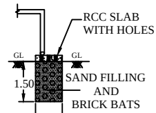
SECTION OF BS
