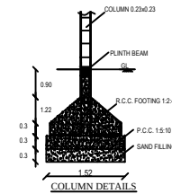
COLUMN DETAILS
