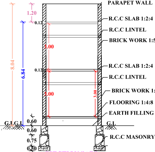
"SECTION AB"
