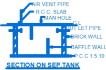
SECTION ON SEP. TANK
