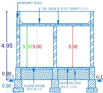
SECTION ON 'AA'
