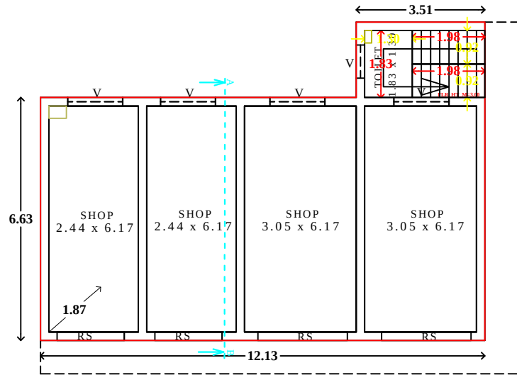
EXG.GROUND FLOOR PLAN
