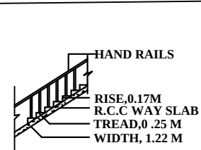
SECTION ON STAIR
