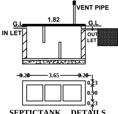
SEPTICTANK DETAILS
