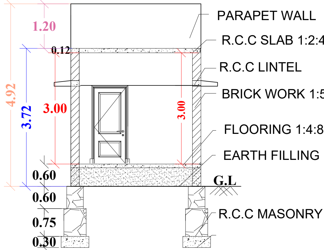
"SECTION "AB"
