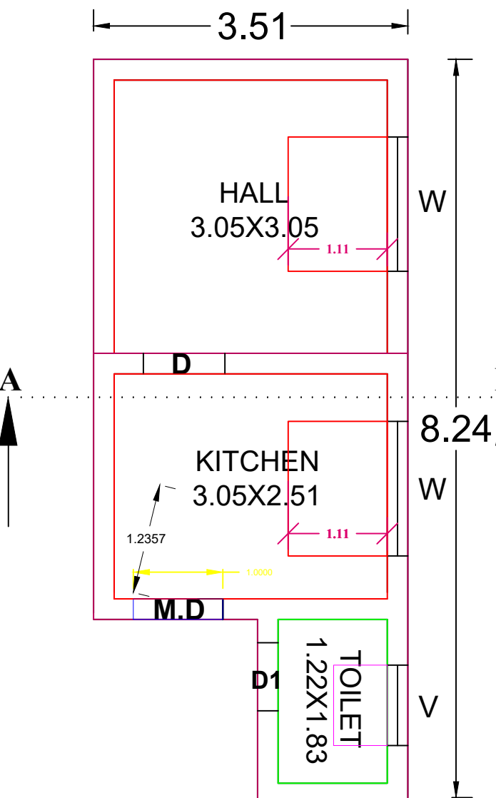
PLAN
