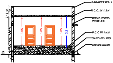
SECTION - "AB"
