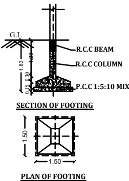
COLUMN DETAILS
