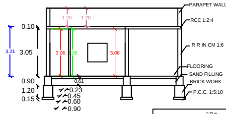
SECTION AB
