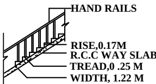
SECTION ON STAIR
