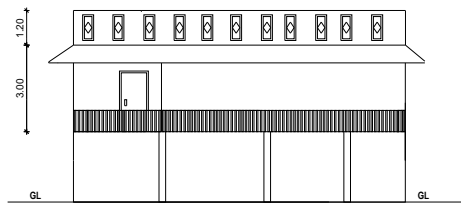
ELEVATION (PROPOSED)
