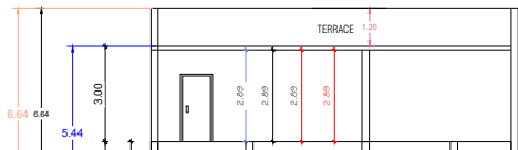
ELEVATION (PROPOSED)
