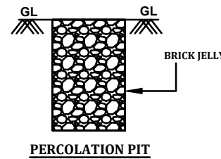
PERCOLATION PIT
