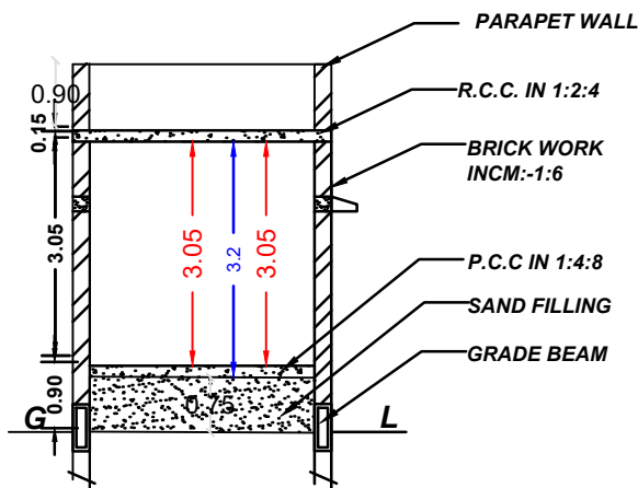
SECTION "AB"
