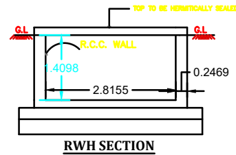
RWH SECTION
