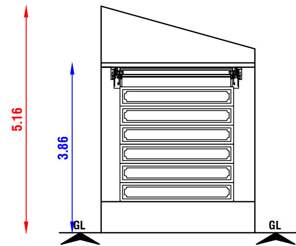
FRONT ELEVATION
