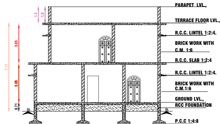
SECTION ON A-A & A'-A'
