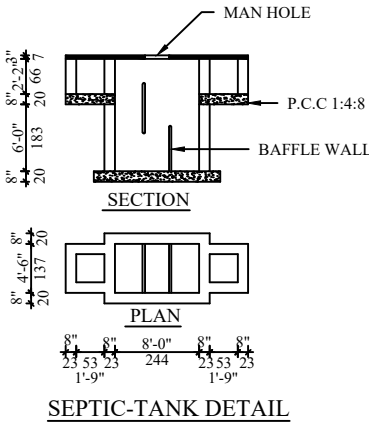
SEPTIC-TANK DETAIL
