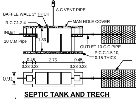
SEPTIC TANK AND TRECH
