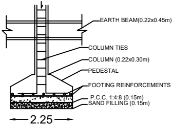
FOUNDATION DETAILS
