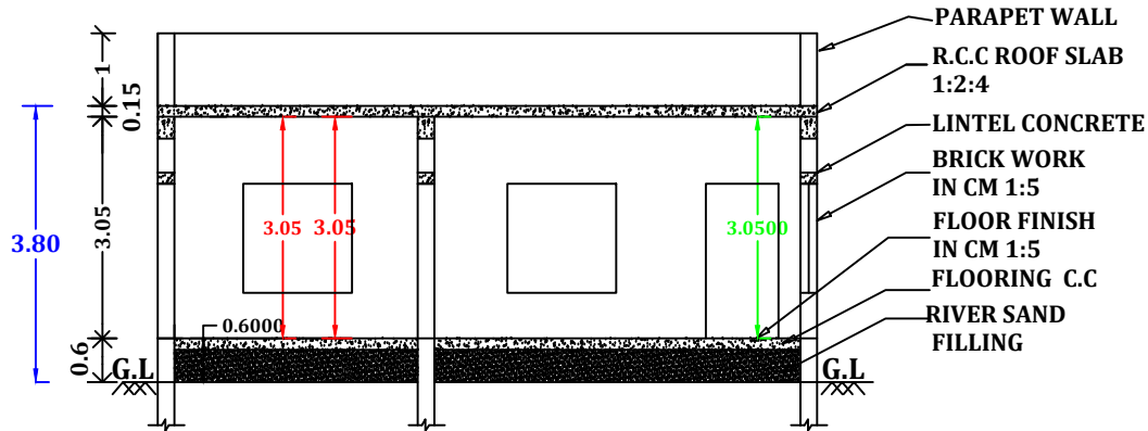
SECTION ON AA1
