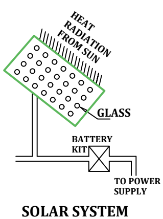
SOLAR SYSTEM
