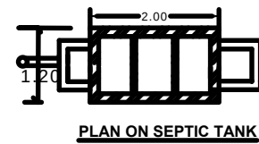
PLAN ON SEPTIC TANK
