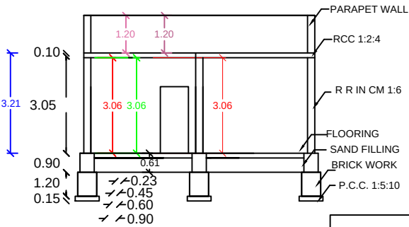
SECTION AB
