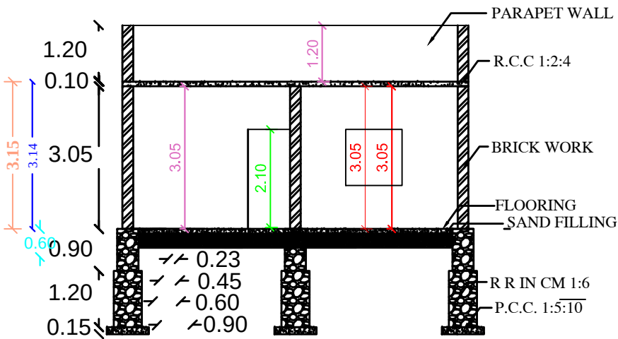
SECTION-AB
