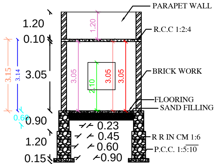
SECTION-AB
