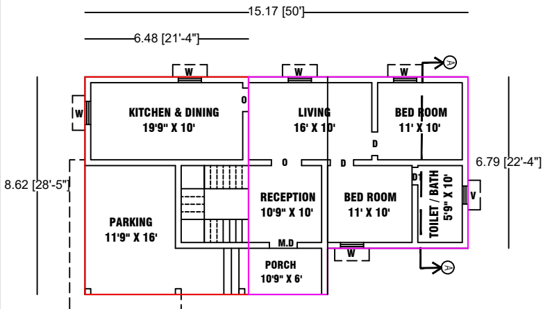
ADDITIONAL & ALTERATION GROUND FLOOR PLAN
