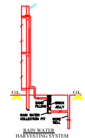
RAIN WATER HARVESTING SYSTEM
