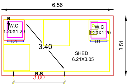
GF PLAN
