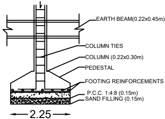
FOUNDATION DETAILS
