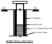
BORE WELL DETAILS
