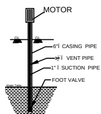
SEC. OF BOREWELL
