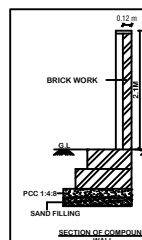
SECTION AB
