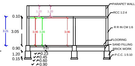
SECTION AB
