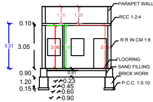
SECTION AB
