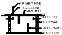
SECTION ON SEP. TANK
