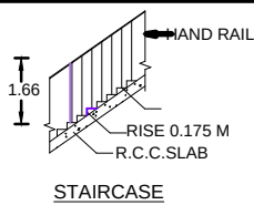
STAIRCASE
