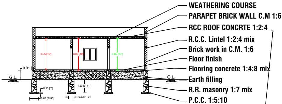
SECTION AB
