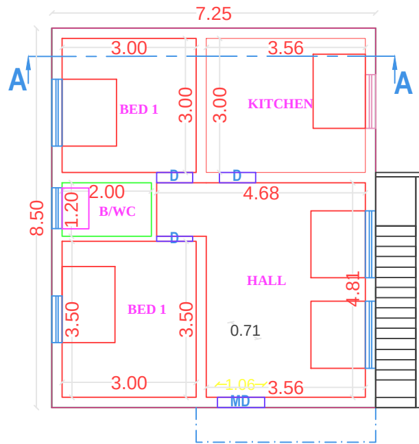
PLAN - GROUND FLOOR ( PROPOSED )
