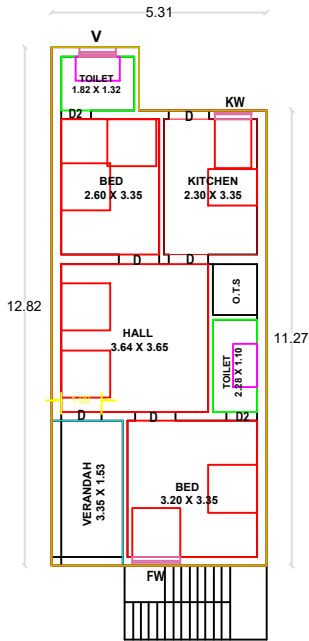
PLAN - GROUND FLOOR ( PROPOSED )
