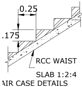
RCC WAIST SLAB 1:2:4 AIR CASE DETAILS
