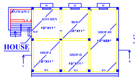
EXG-GROUND FLOOR PLAN DOOR NO:0/3/274 SHOPS(I-III) & HOUSE-1
