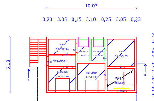
HOUSE-I HOUSE-II EXG- FIRST FLOOR PLAN DOOR NO:3/274-1 &3/274-2
