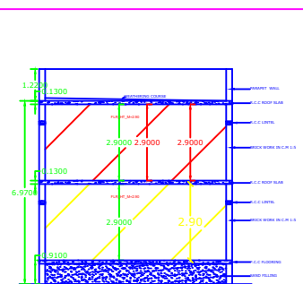
EXG-SECTION ON A-A
