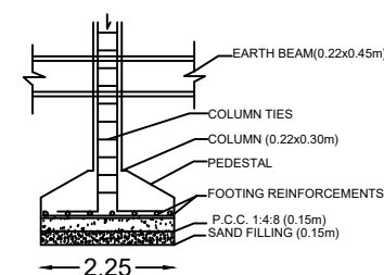
FOUNDATION DETAILS
