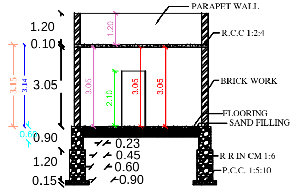
SECTION-AB
