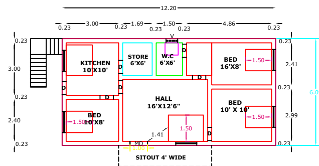
PRO GROUND FLOOR RESIDENTIAL PLAN
