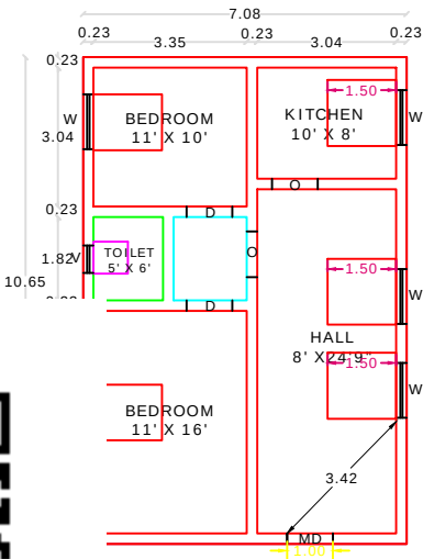
GROUND FLOOR DENTIAL PLAN
