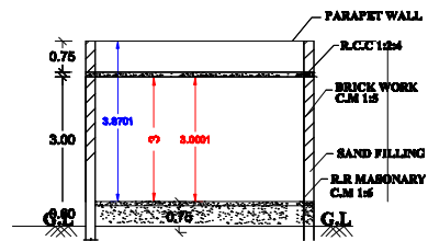
SECTION ON "BB"
