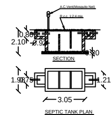
SEPTIC TANK PLAN
