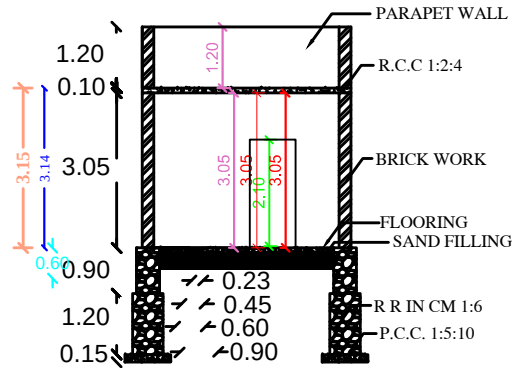
SECTION-AB
