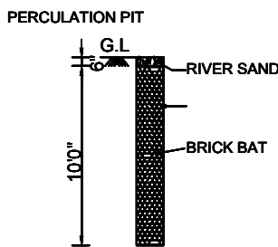
PERCOLATION PIT
