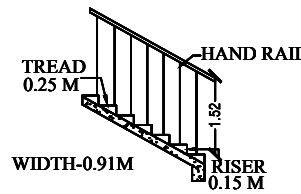
STAIRCASE DETAILS
