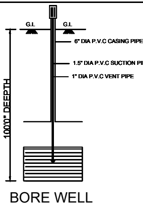
BORE WELL
