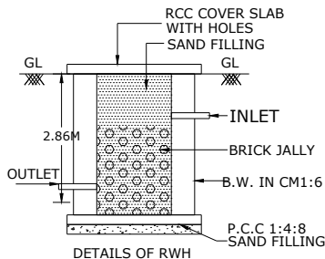
DETAILS OF RWH
