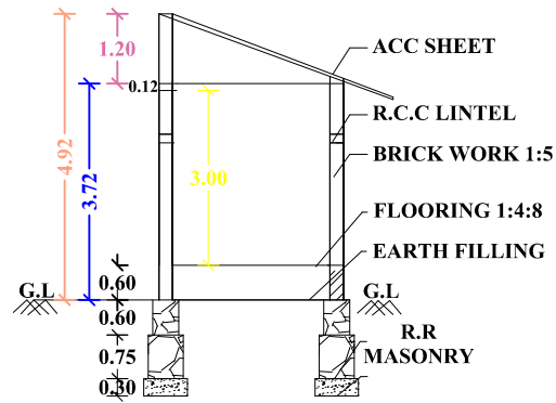
"SECTION AB"
